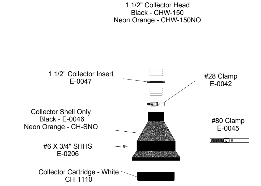
FIGURE 4 - Collector Head
