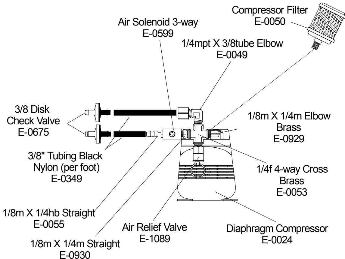
FIGURE 10 - BOOM TRACKER Model BTD Compressor Assembly
