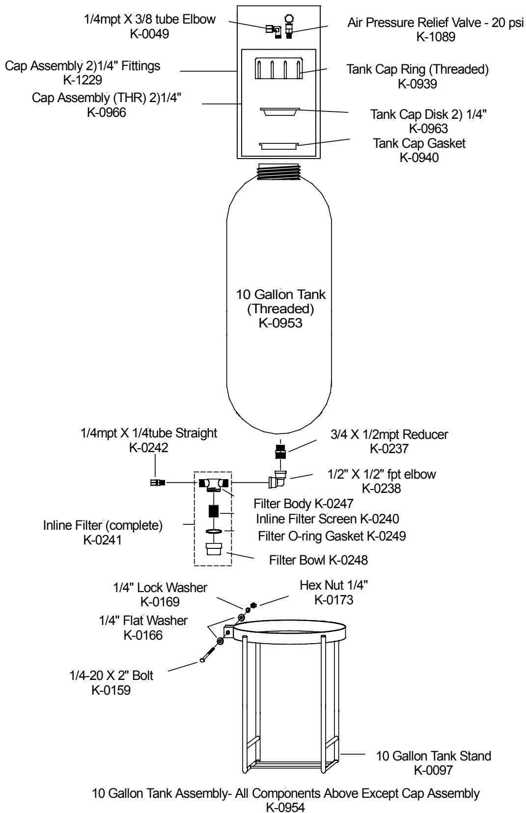
FIGURE 13 - BOOM TRACKER Tank 10 Gallon
