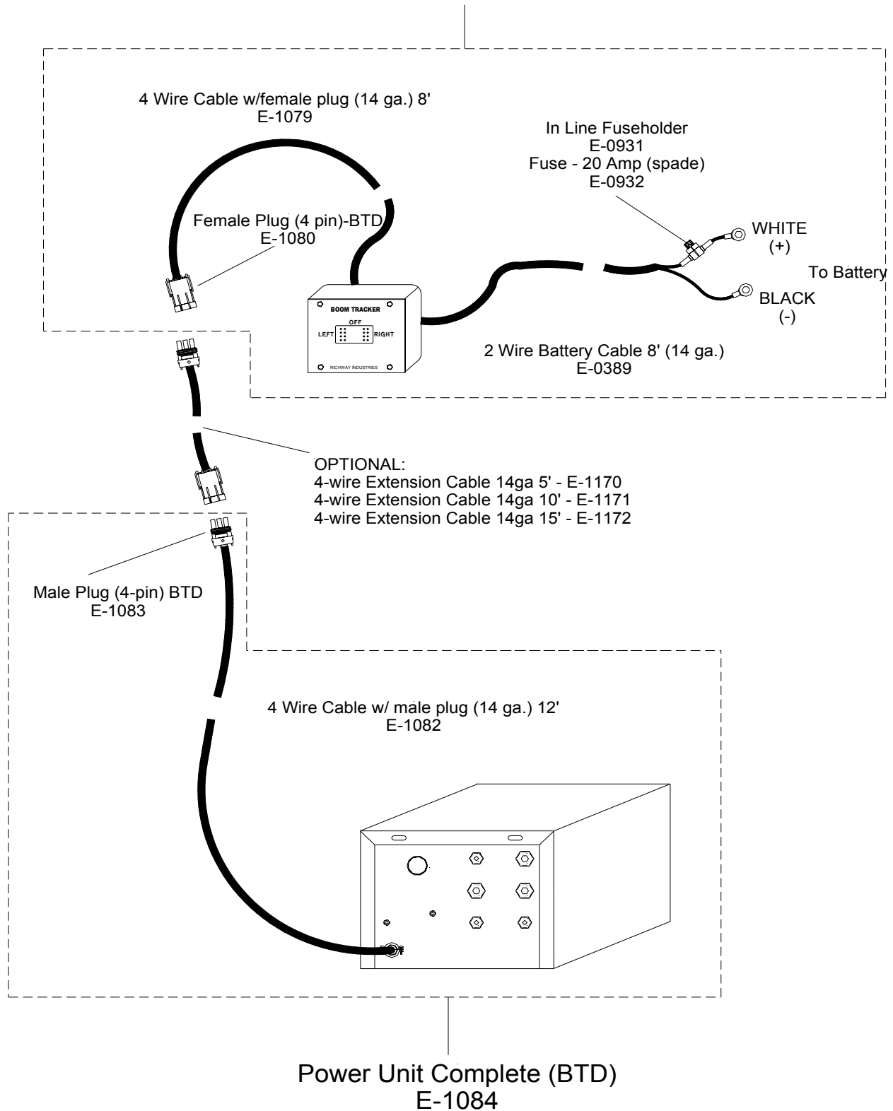
FIGURE 7 - BOOM TRACKER Model BTD Wiring
