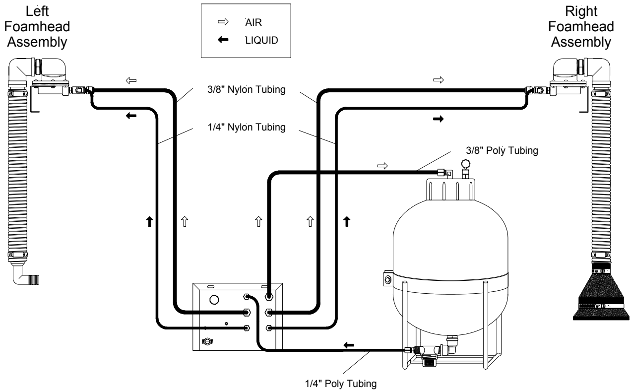
FIGURE 5 - BOOM TRACKER Model BTD Liquid and Air Flow
