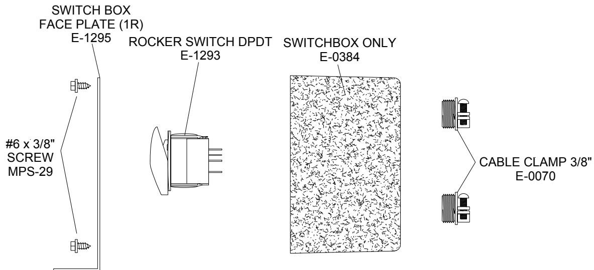
FIGURE 6 - BOOM TRACKER Model BTD Switch Box
