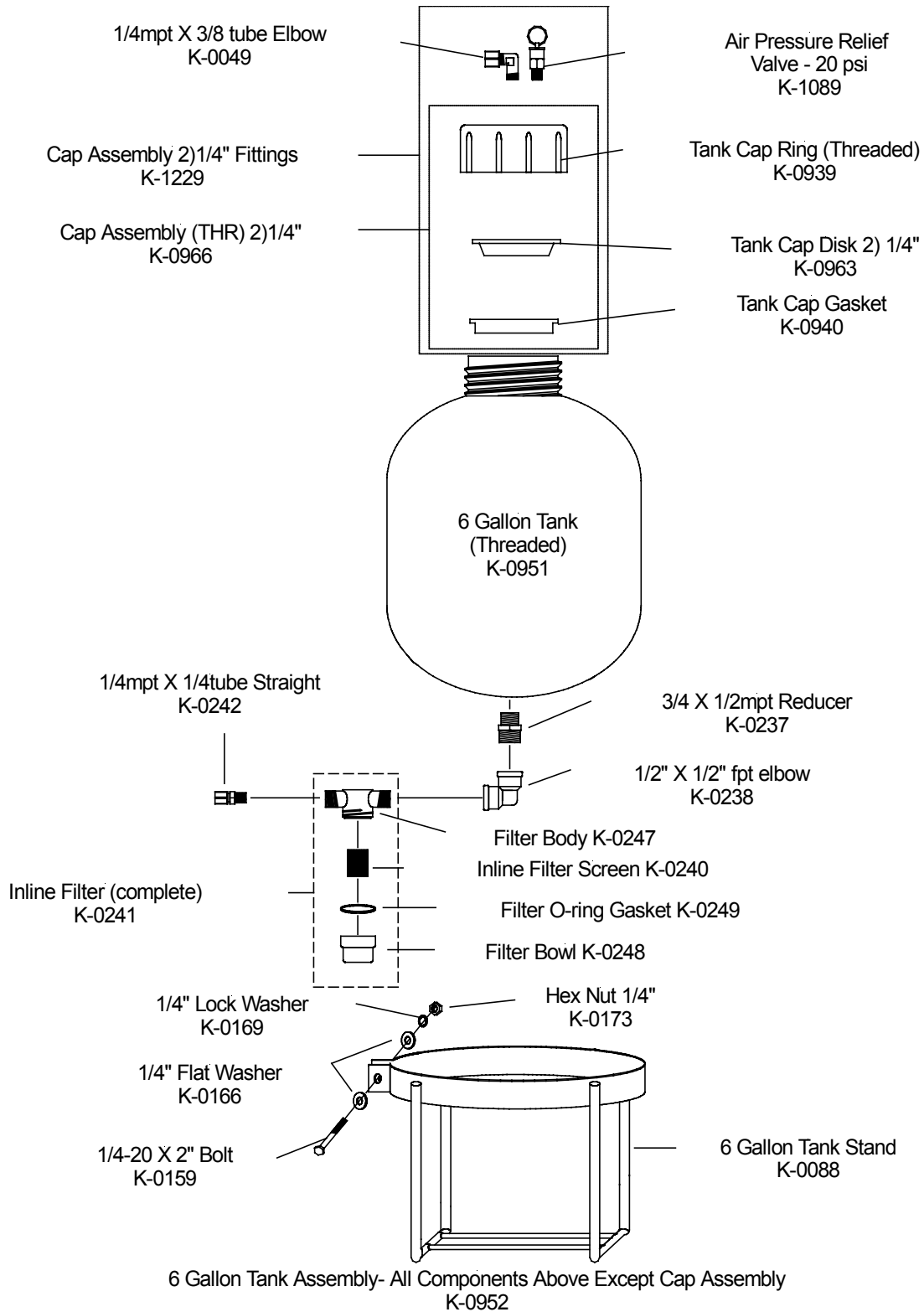
FIGURE 12 - BOOM TRACKER Tank 6 Gallon
