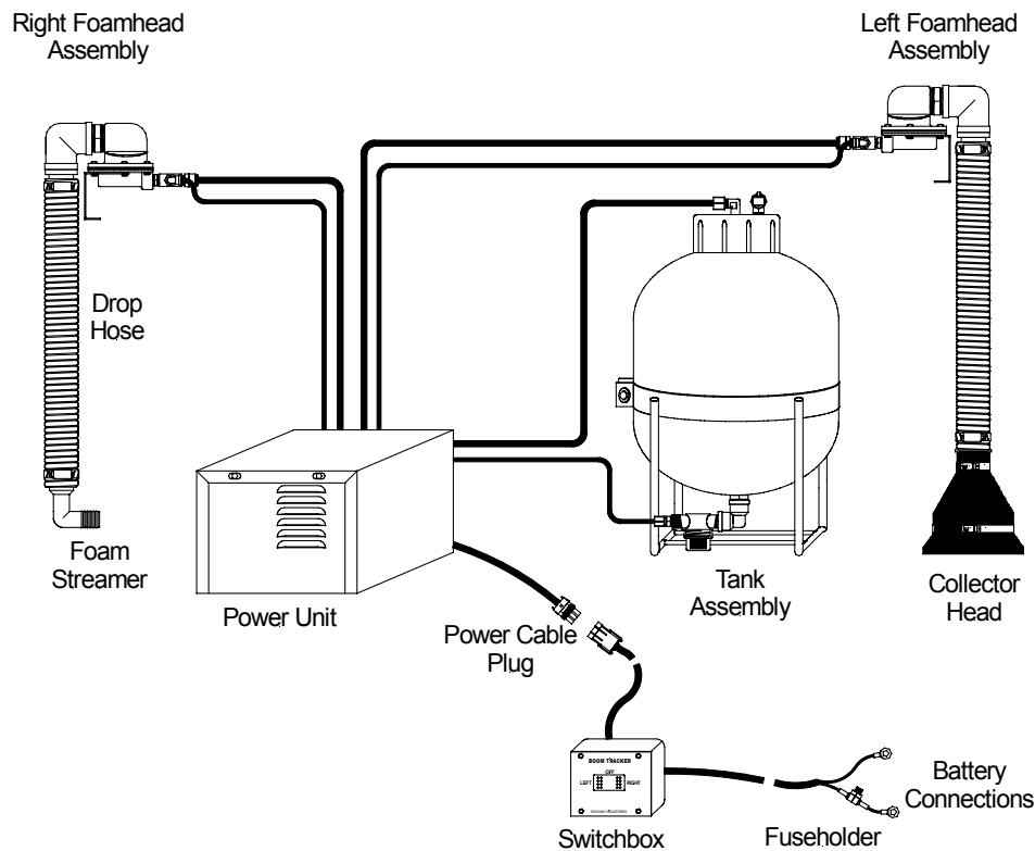
FIGURE 1 - BOOM TRACKER Model BTD-2060 Foam Marker
