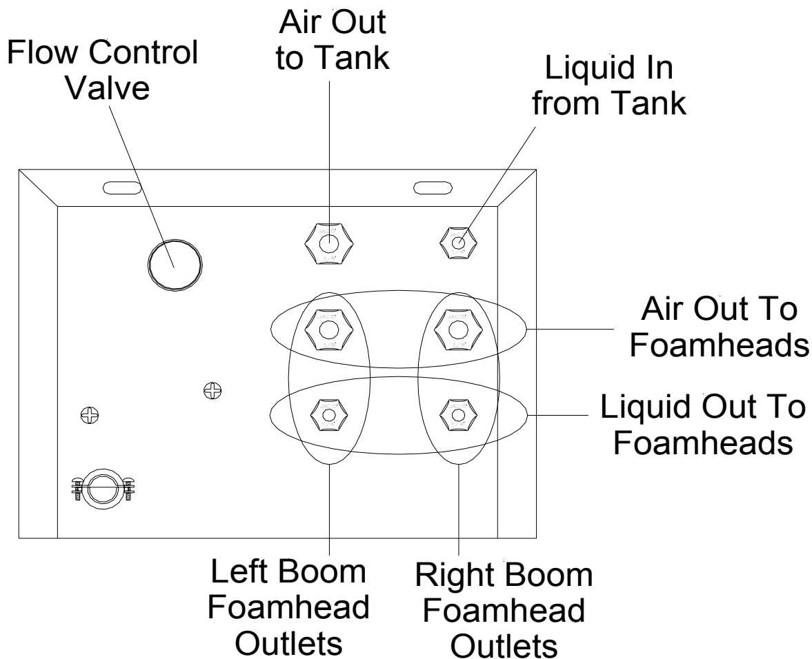
FIGURE 2 - BOOM TRACKER Model D Power Unit
