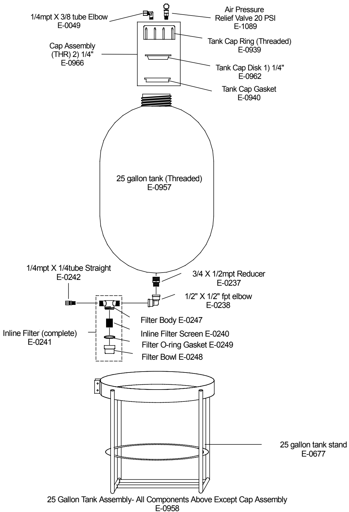
FIGURE 15 - BOOM TRACKER Tank 25 Gallon
