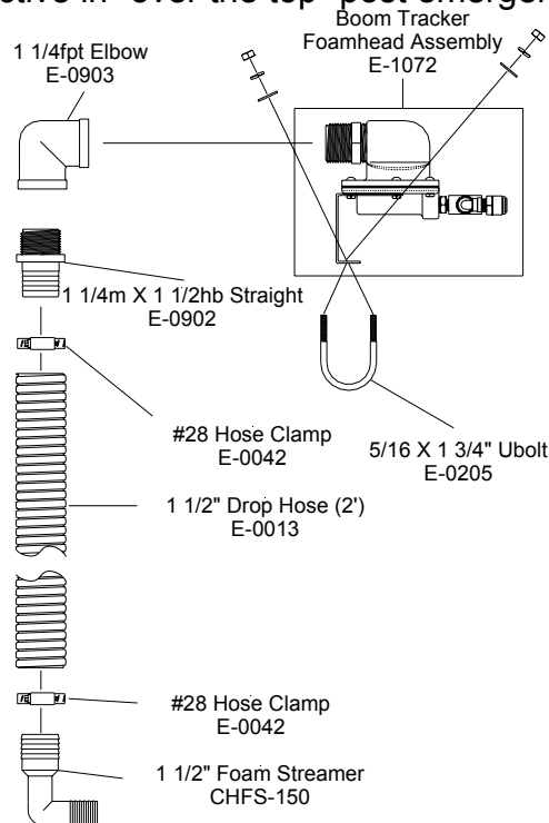
FIGURE 3 - BOOM TRACKER Foam Head and Boom End Assembly
