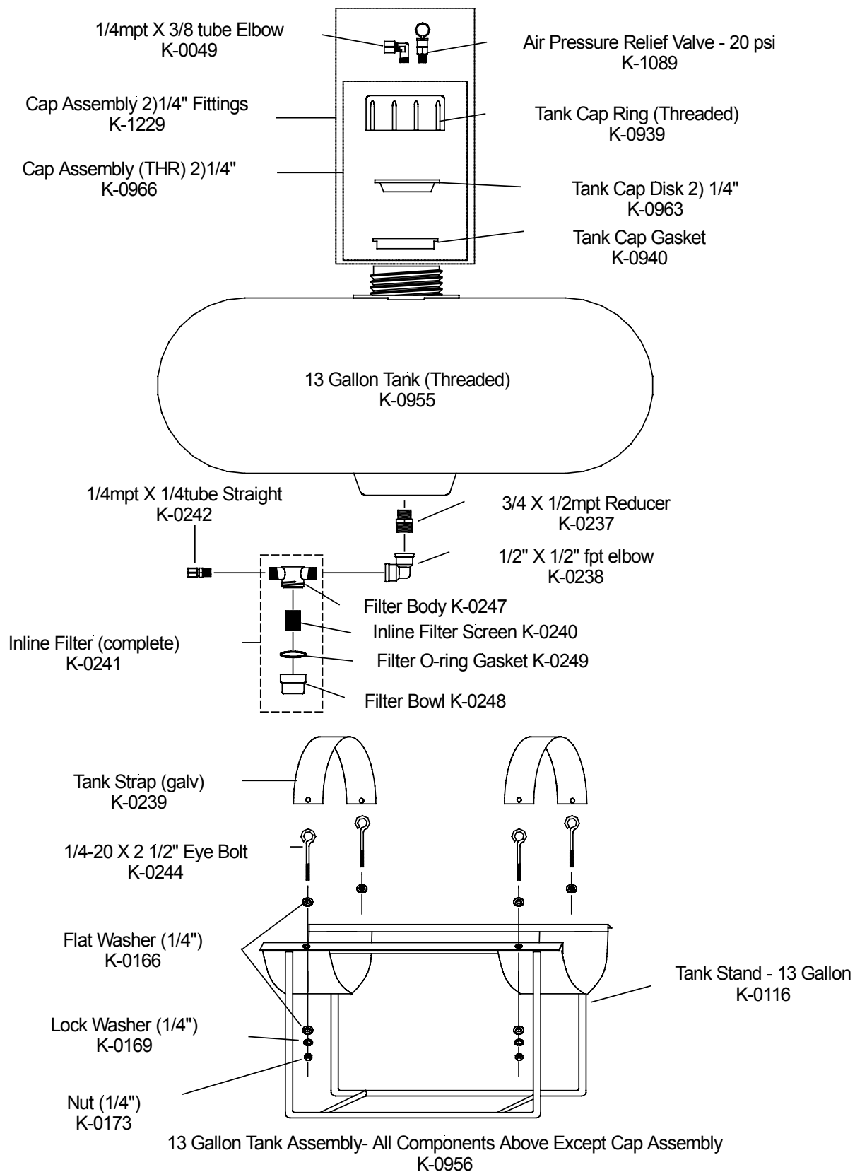
FIGURE 14 - BOOM TRACKER Tank 13 Gallon
